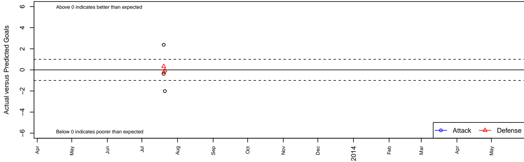
Pateadores MV B95 Dots are actual minus expected GF (blue circles) and GA (red triangles). Blue line is smoothed change in attack strength. Red is smoothed change in defense strength.
